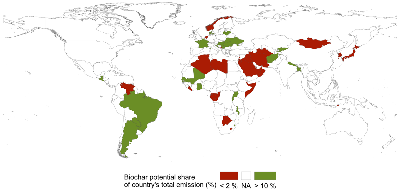
Fig. 7 Global map of countries with highest potential biochar impact (> 10% of national emissions; green) and lowest potential biochar impact (< 2% of national emissions; red)
