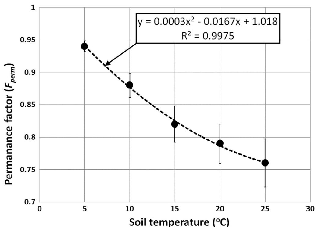
Fig. 1 100-year biochar permanence factor as a function of soil temperature, assuming biochar production via pyrolysis at high temperature ( \geq 600 °C); based on data from Woolf et al. (2021). The bars indicate the standard errors reported in Table 5 of the same publication
