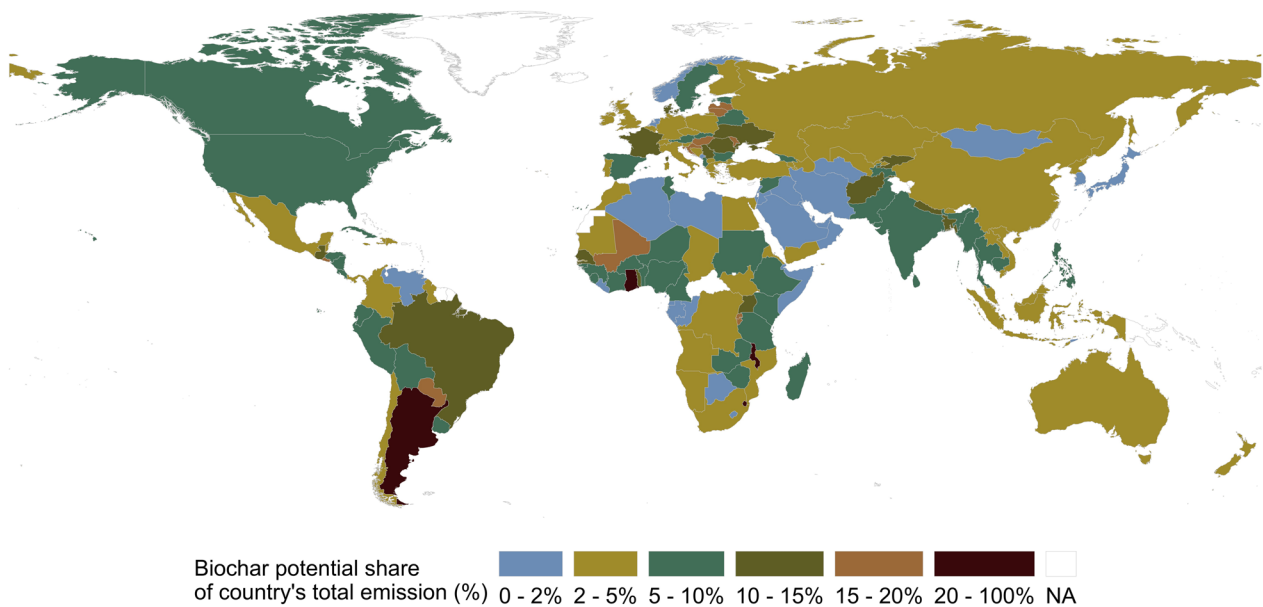
Fig. 6 Global biochar carbon dioxide removal potential map as a percentage of total national GHG emissions
