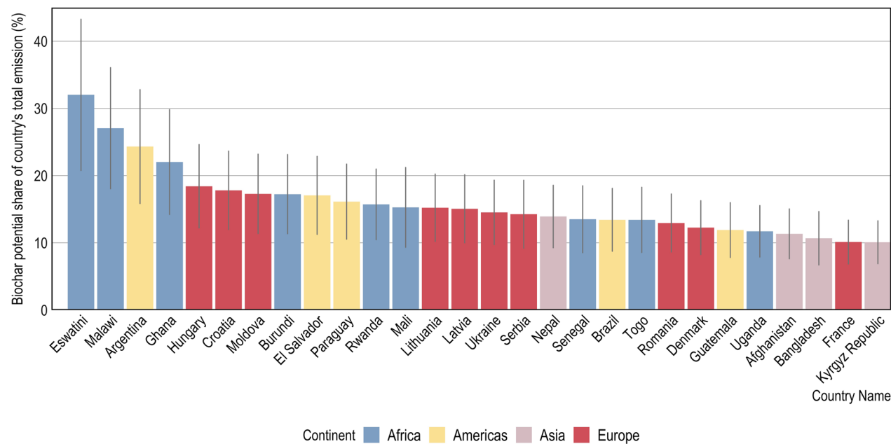
Fig. 5 Countries with the largest biochar carbon dioxide removal potential as percentage of total GHG emissions. Presented data are for the 28 countries with biochar carbon dioxide removal > 10% of total national emissions. Error bars represent standard deviation computed via Monte Carlo simulation (Methods section and Additional file 2)
