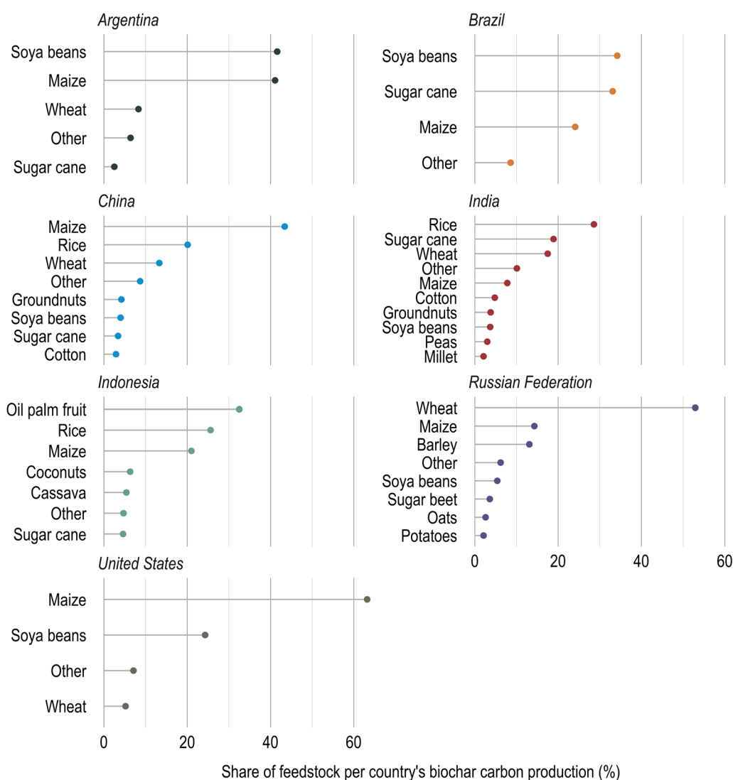
Fig. 8 Major sources of crop residues in high biochar potential countries, based on the percentage of biochar carbon production
