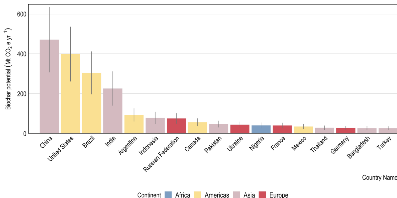
Fig. 3 Countries with the largest biochar carbon dioxide removal potential (Mt CO 2 e year -1 ). Presented data are for the 17 countries with biochar carbon dioxide removal potential > 25 Mt CO 2 e year -1 . Error bars represent standard deviation computed via Monte Carlo simulation (Methods section and Additional file 2)
