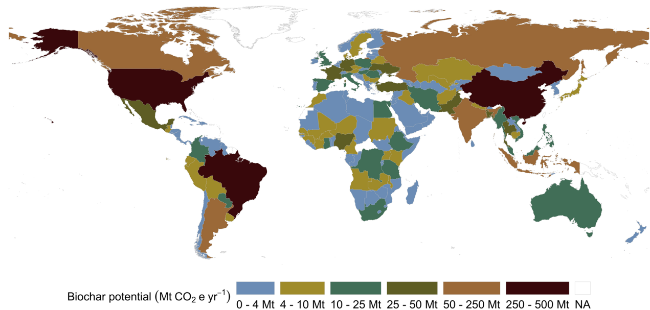
Fig. 4 Global biochar carbon dioxide removal potential map ( \text{Mt CO}_2\text{e year}^{-1} )
