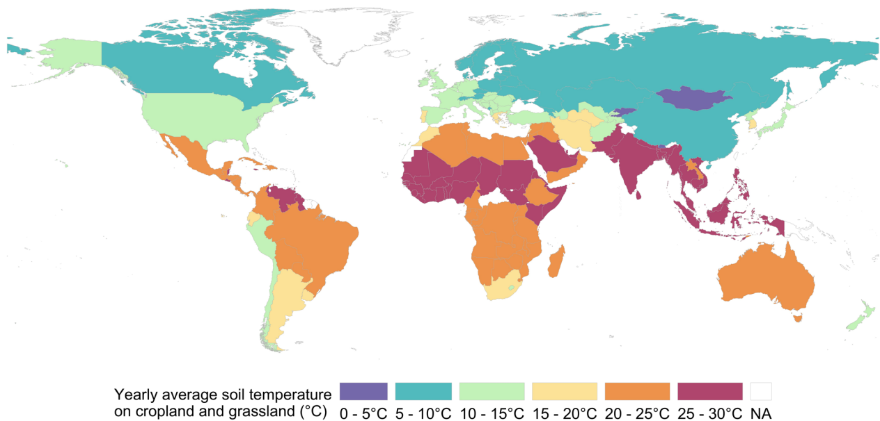
Fig. 2 National average soil temperature on croplands and grasslands for computation of biochar permanence factor
